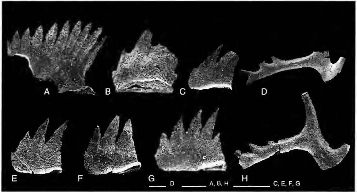
FIG. 5. — Spathian conodonts from the TNK-R-09. A, Neospathodus triangularis (Bender), B, C, Cornudina igoi Koike; D, H, Neohindeodella benderi (Kozur & Mostler); E, F, Neospathodus sp.; G, ? Neospathodus clinatus Orchard & Sweet. Scale bars: 100 µm.
